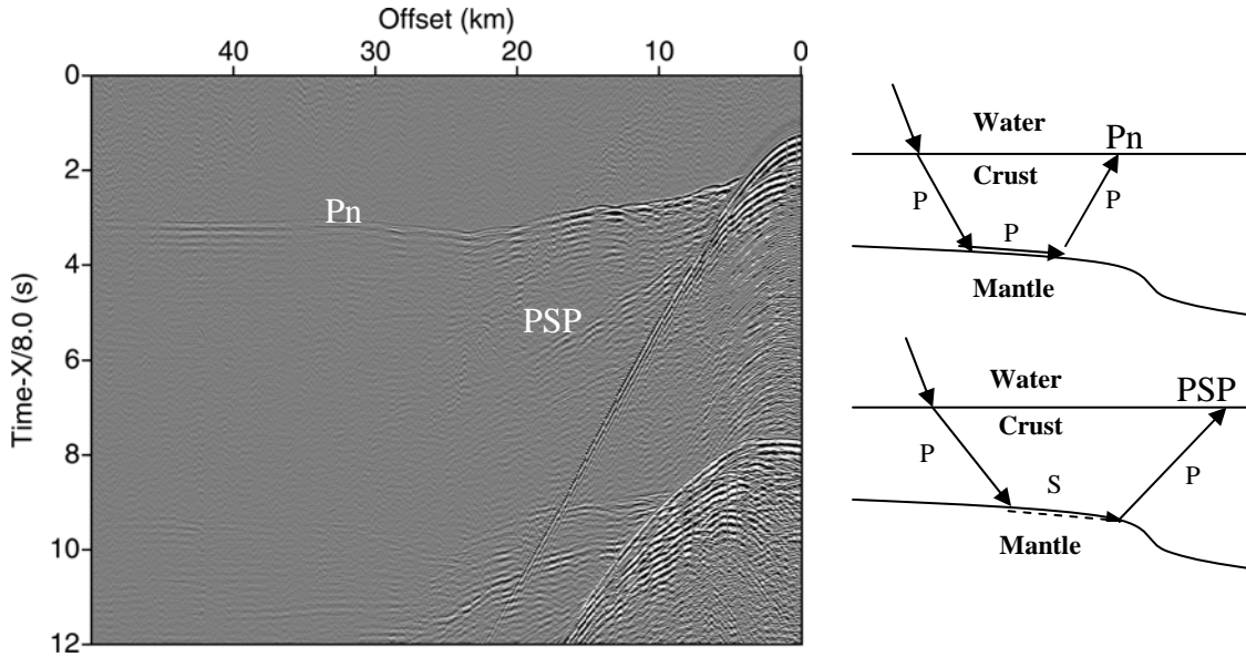
Figure 16. An example OBS data. Vertical component is shown. Two major refraction arrivals are Pn (refracted in the subducting slab) and PSP (refracted shear wave). Right diagram shows the ray-paths of the two different arrivals. The incident P-wave mode of PSP arrival in the crust has very likely been converted into shear-mode before it arrives at the crust-mantle boundary.
